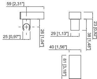
ABS minimalist hand shower support Soporte de ducha minimalista en ABS
