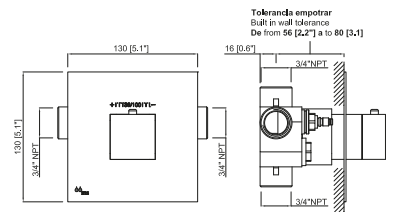
Anti limescale thermostatic cartridge Cartucho termostático anticalcáreo
