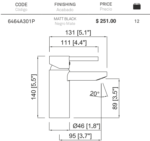
Single lever lavatory Monomando de lavabo
