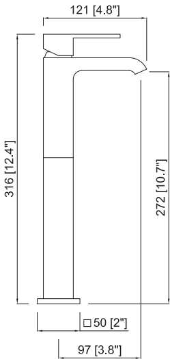
WATERFALL single lever with high profile Monomando de lavabo WATERFALL abierto con prolongador
