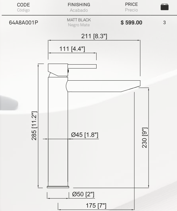
Single lever with high profile 6,70" spout Monomando de lavabo alto con caño de 17 cm
